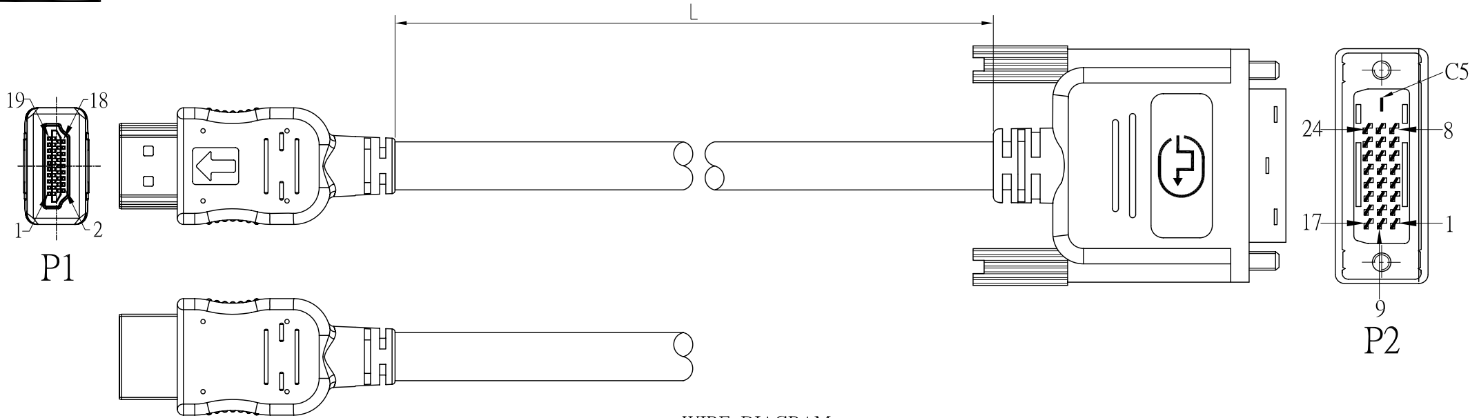
WIRE DIAGRAM
